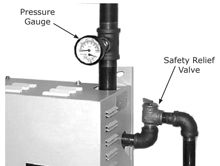
Figure 1A - Safety Relief Valve
