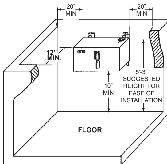
Figure 1 - BOILER LOCATION & CLEARANCE DIMENSIONS
