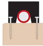
3/8" Flush Mount Clip for use on pipe or tubing with ID of 3/8" Product Code: F4OD
